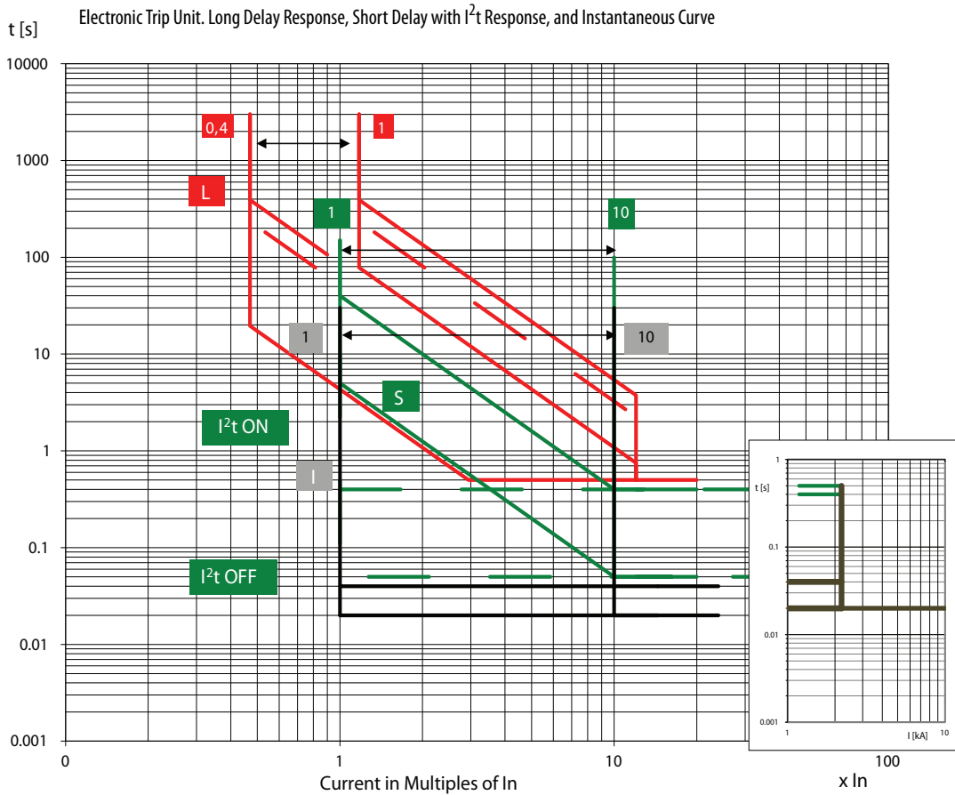
Figure 16 - Time-current Curves for Bulletin 140G-H Thermo-magnetic Molded Case Circuit Breaker, 600V AC (50/60 Hz), 25 A, 60 A, 100 A, 125 A
