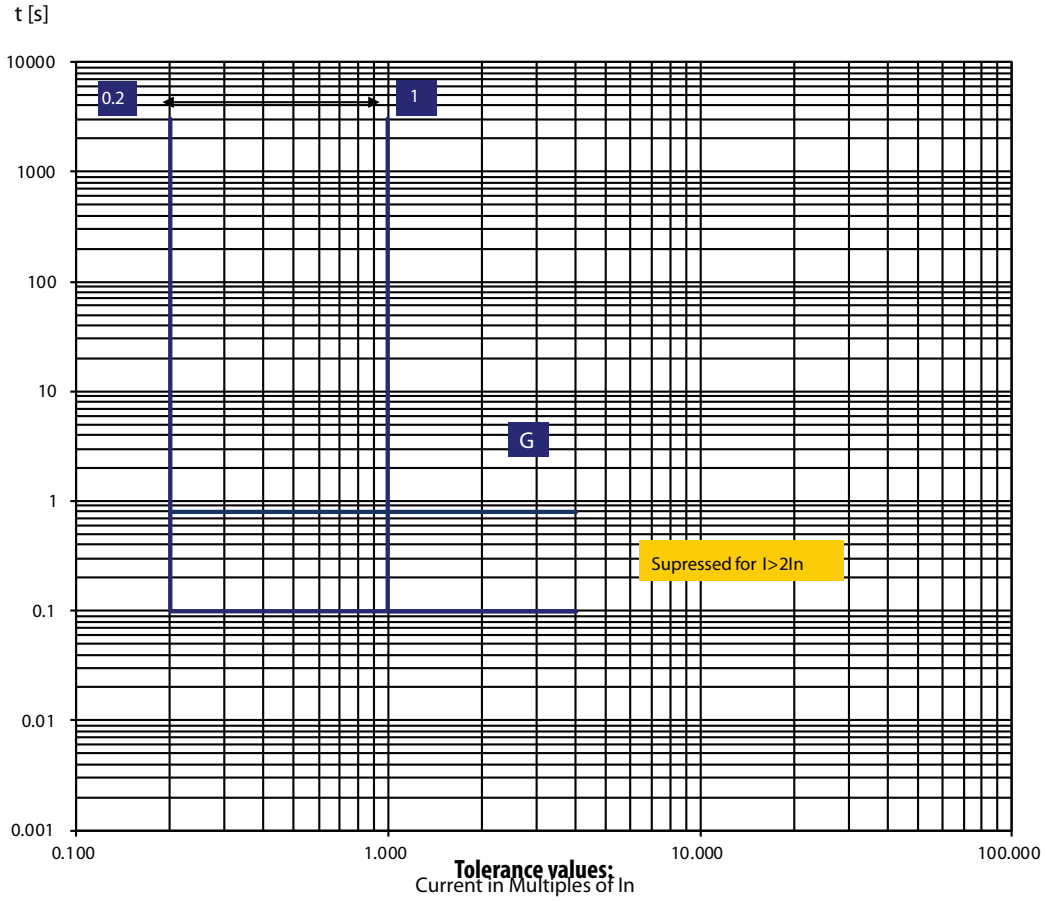
Figure 17 - Time-current Curves for Bulletin 140G-H Thermo-magnetic Molded Case Circuit Breaker, Ground Fault Protection Curve, 600V AC (50/60 Hz), 25 A, 60 A, 100 A, 125 A
