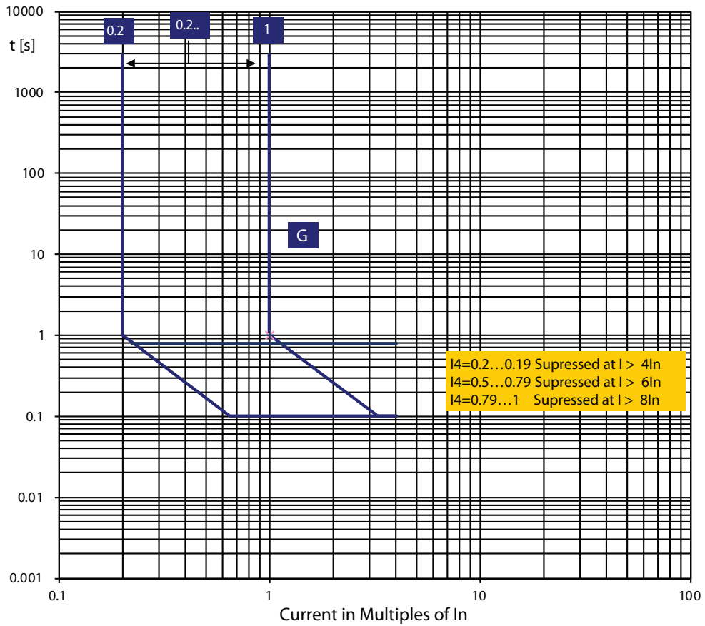
Figure 27 - Time-current Curves for Bulletin 140G-K Molded Case Circuit Breaker, Ground Fault Protection Curve, 600V AC, (50/60 Hz) 300 A, 400 A
