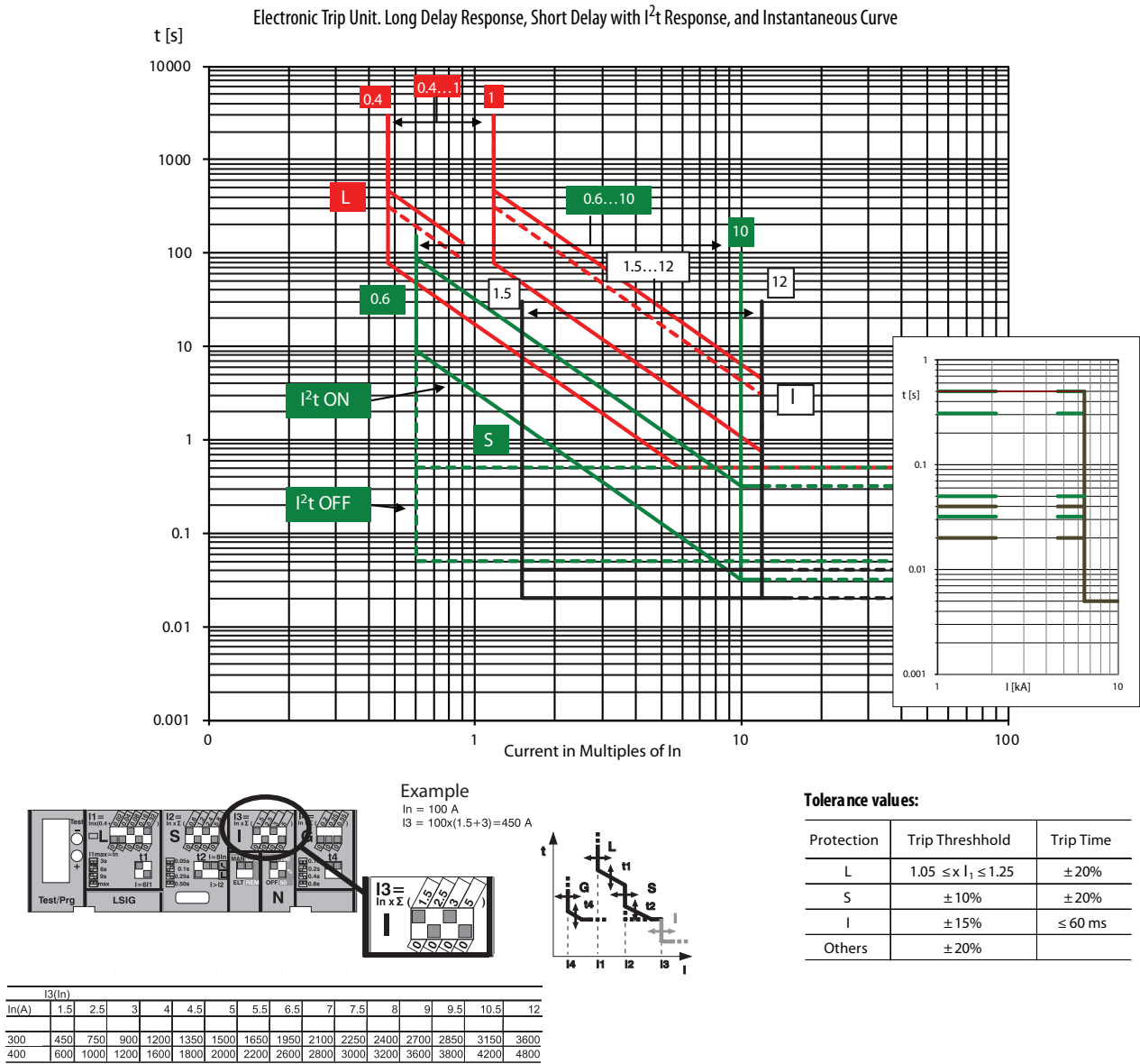
Figure 26 - Time-current Curves for Bulletin 140G-K Molded Case Circuit Breaker, 600V AC, (50/60 Hz) 300 A, 400 A
