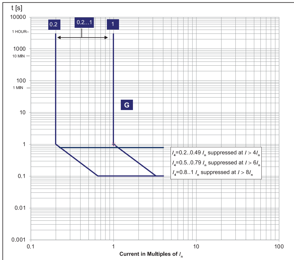
Ground Fault Protection Curve for LSI G MCCBS
