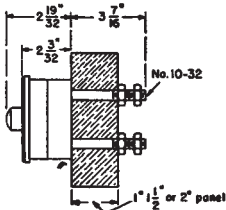
Fig. 5. 4- or 6-pole surface mounted on 1- to 2-in panel
