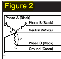
Figure 2 WYE 3 Phases, 1 Neutral, 1 Ground
