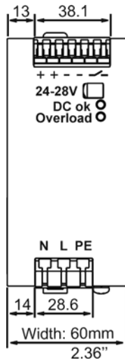
Fig. 23-1 Front view
