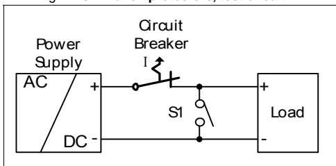
Fig. 27-3 Branch protectors, test circuit 1
