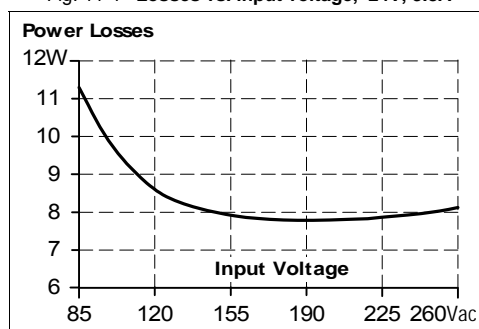
Fig. 11-4 Losses vs. input voltage, 24V, 3.8A
