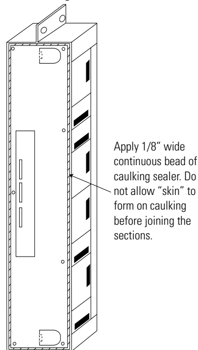
Figure 1 Correct Application of Caulking
