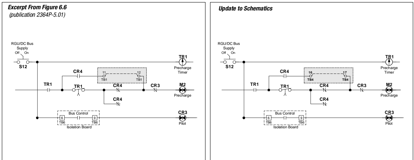
Figure 1 Updates to RGU Schematics—Parallel Configuration
