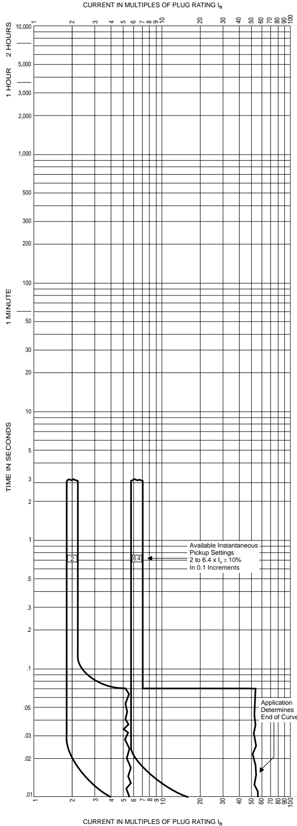
Circuit Breaker Time/Current Curves (Phase Current) Series C ® R - Frame Circuit Breakers Equipped With 2500A Digitrip Optim Trip Units Response: INSTANTANEOUS AND OVERRIDE
