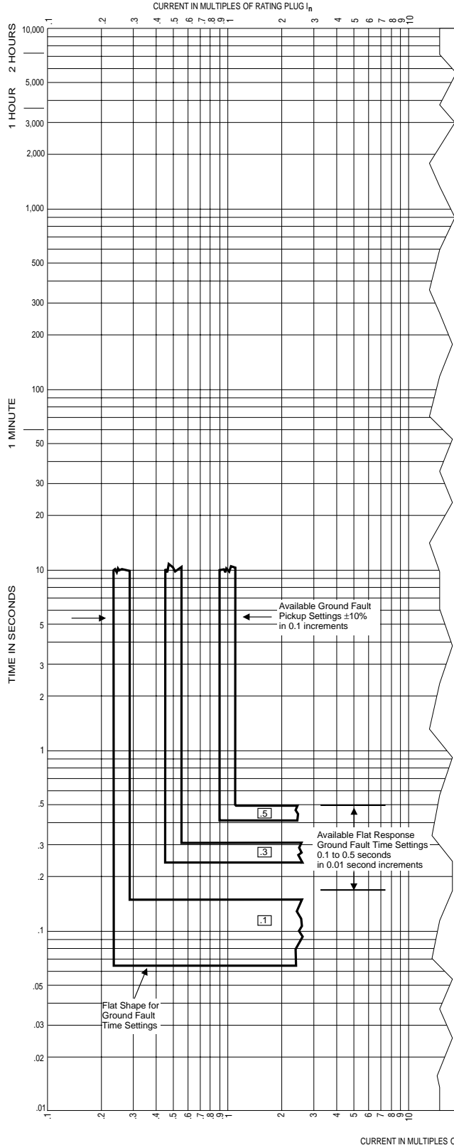
Circuit Breaker Time/Current Curves (Ground Current) Series C® R - Frame Circuit Breakers Equipped With 2000A Digitrip Optim Trip Units Response: GROUND FAULT TRIP OR GROUND FAULT ALARM ONLY
