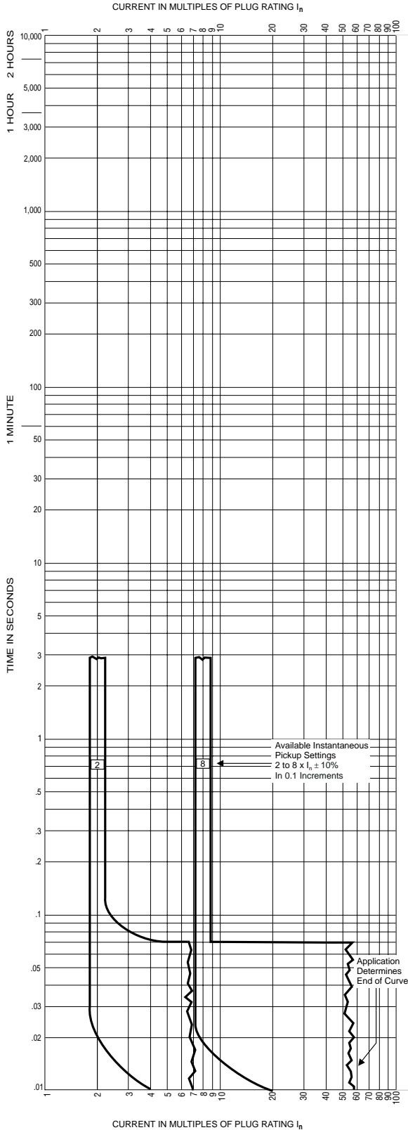
Circuit Breaker Time/Current Curves (Phase Current) Series C® R - Frame Circuit Breakers Equipped With 2000A Digitrip Optim Trip Units Response: INSTANTANEOUS AND OVERRIDE
