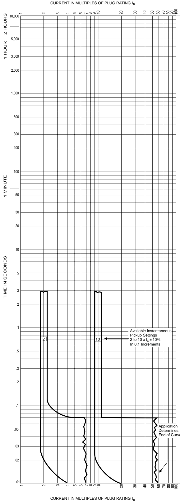
Circuit Breaker Time/Current Curves (Phase Current) Series C ® R - Frame Circuit Breakers Equipped With 1600A Digitrip Optim Trip Units Response: INSTANTANEOUS AND OVERRIDE
