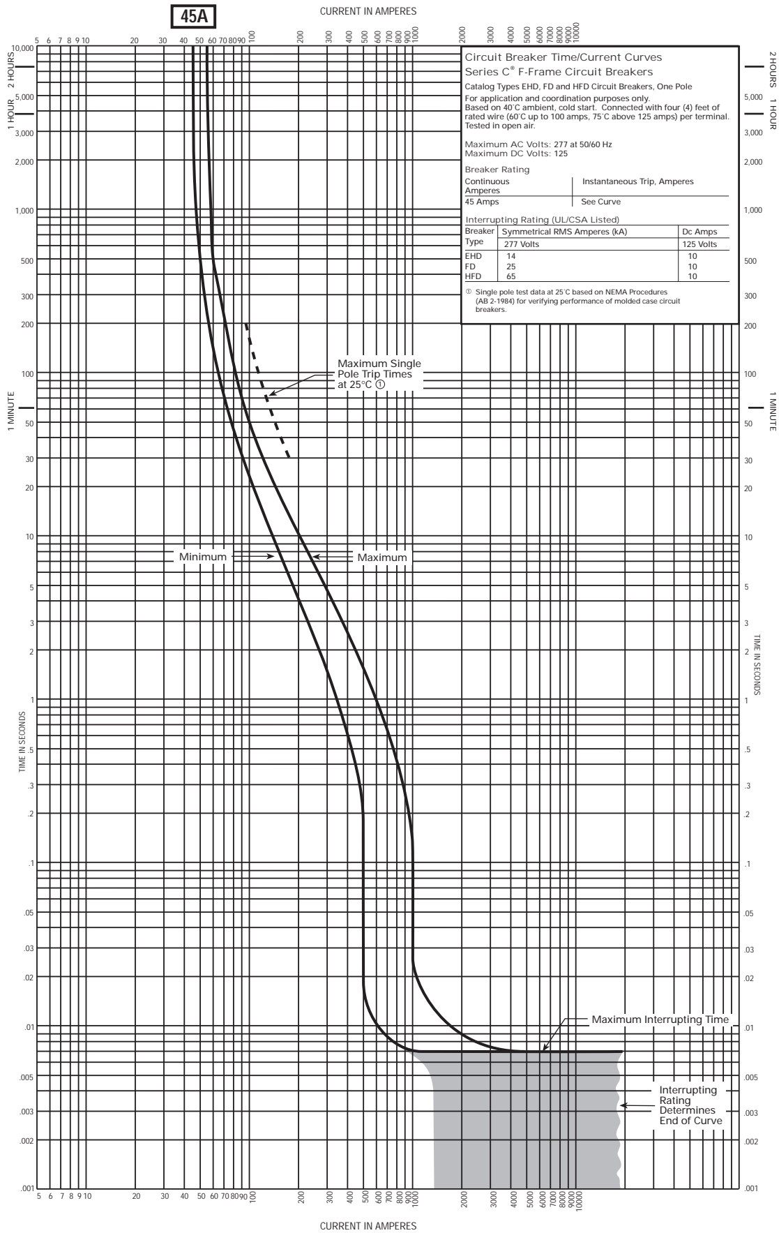
FIGURE 7. TYPES EHD, FD AND HFD 45 AMPERES — CURVE NO. SC-4429-88A
