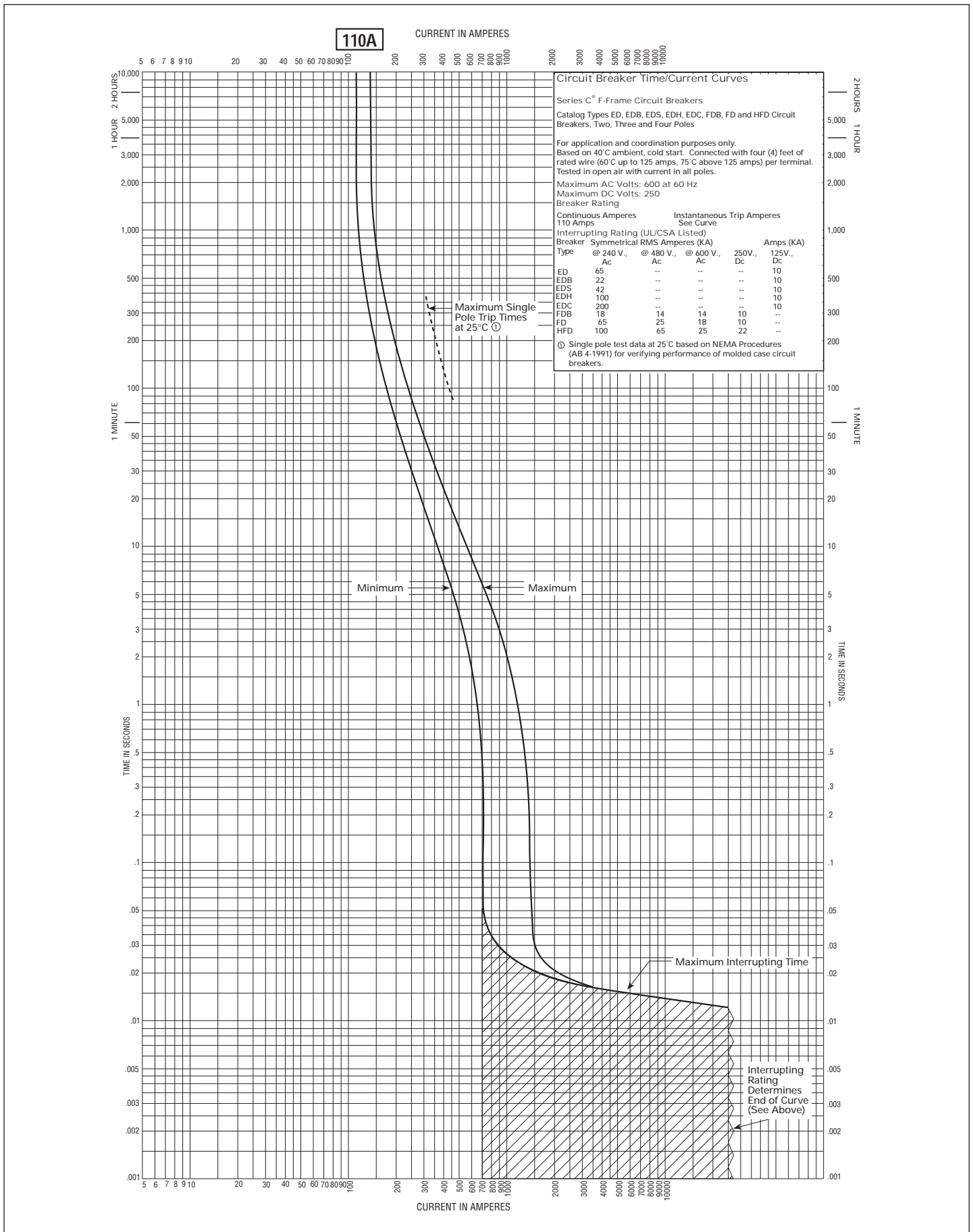
FIGURE 30. TYPES ED, EDB, EDS, EDH, EDC, FDB, FD AND HFD 110 AMPERES — CURVE NO. SC-4147-87B
