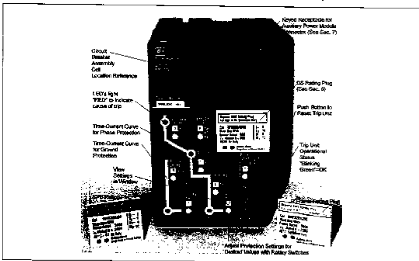
Fig. 1 Digitrip RMS 510 Trip Unit Model LSiG with Rating Plug
