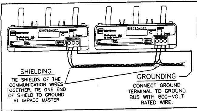
Fig. 4 Network Interwiring
