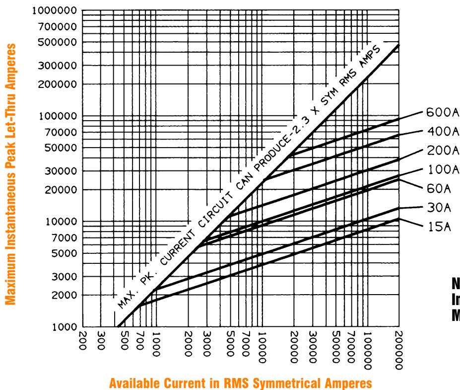
Peak Let-Through Current Data — TRS15 to 600, 600 Volts AC
