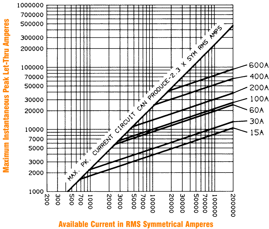
Peak Let-Through Current Data — TR30 to 600, 250 Volts AC
