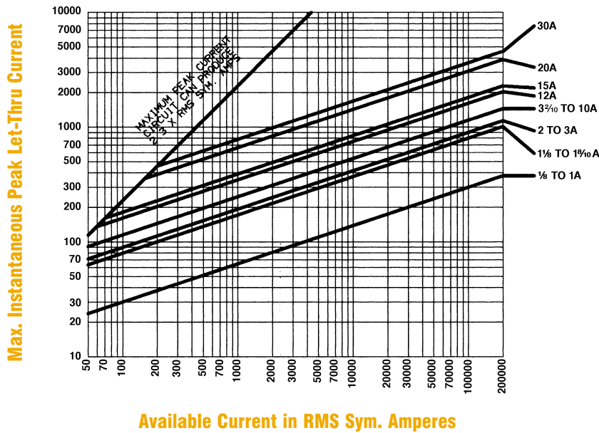
Peak Let-Thru Current Data – ATQR1/8 to 30, 600 Volts AC
