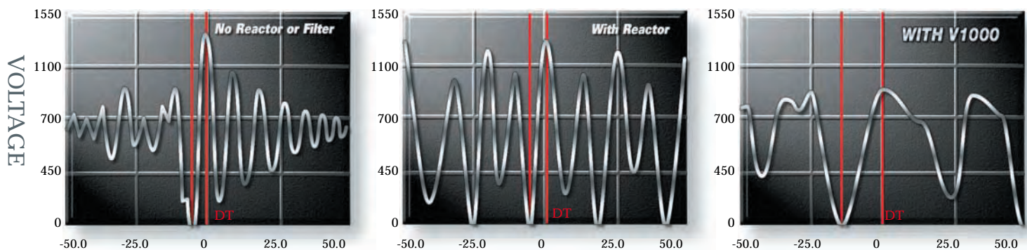
Carrier Frequency 8KHZ; 500 Feet of Cable Rate of voltage rise at motor terminals
